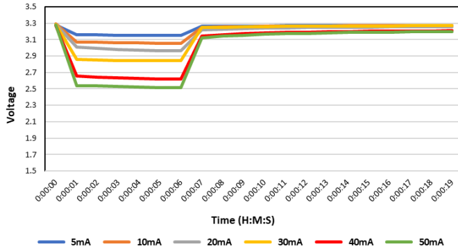
Pulse Load Capability (5 sec load)
